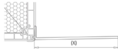
INNEN – x = 20-120 mm in 5 mm Schritten 119.393 Preis: 6,80 €/m
